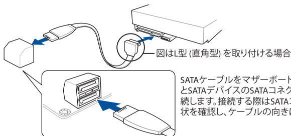
PRIME X399-A Serial ATA 6.0Gb/s connectors
